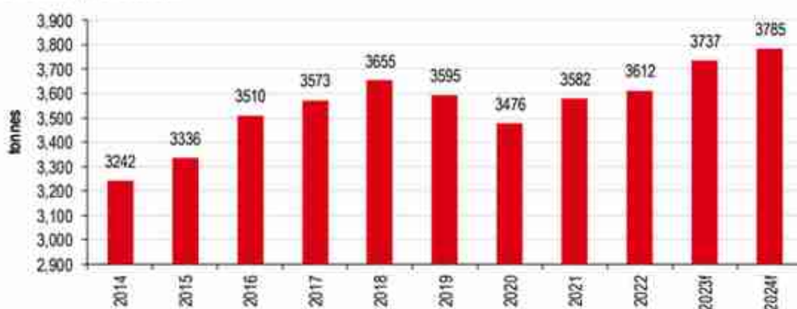
13. Mine production
